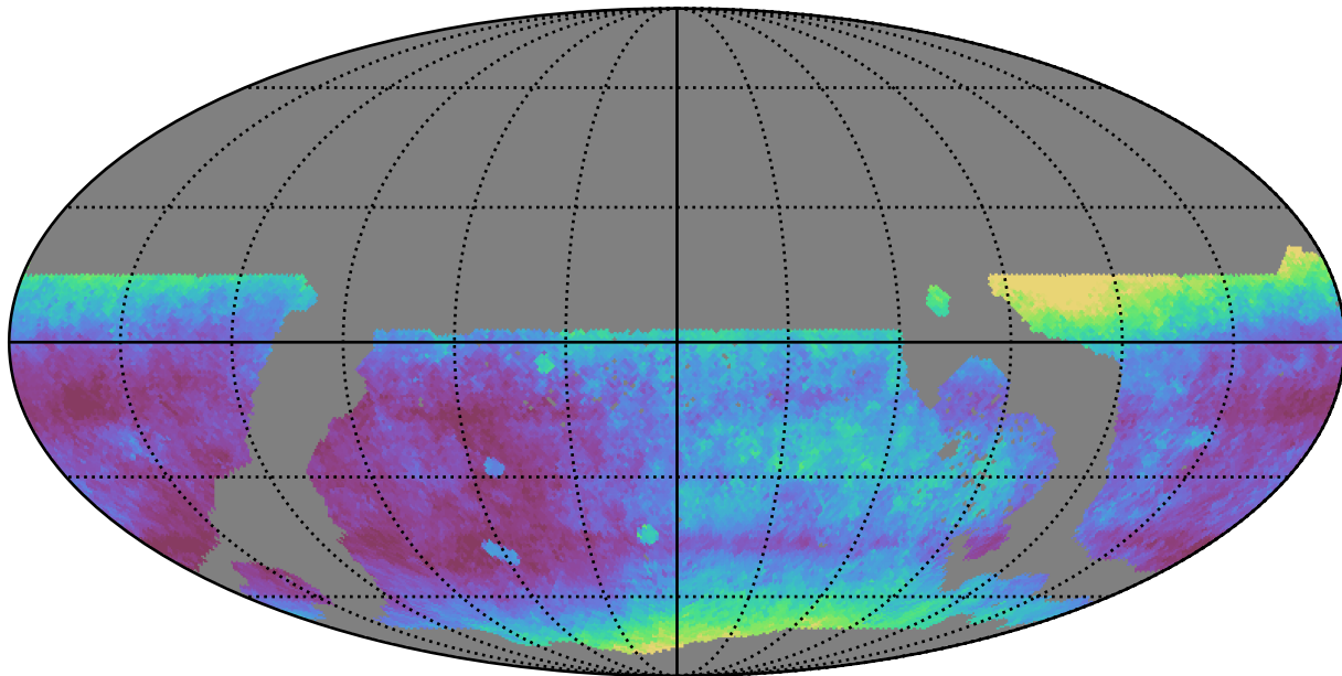
weather_cloudso1v3.4_10yrs WFD r band: Median seeingEff
