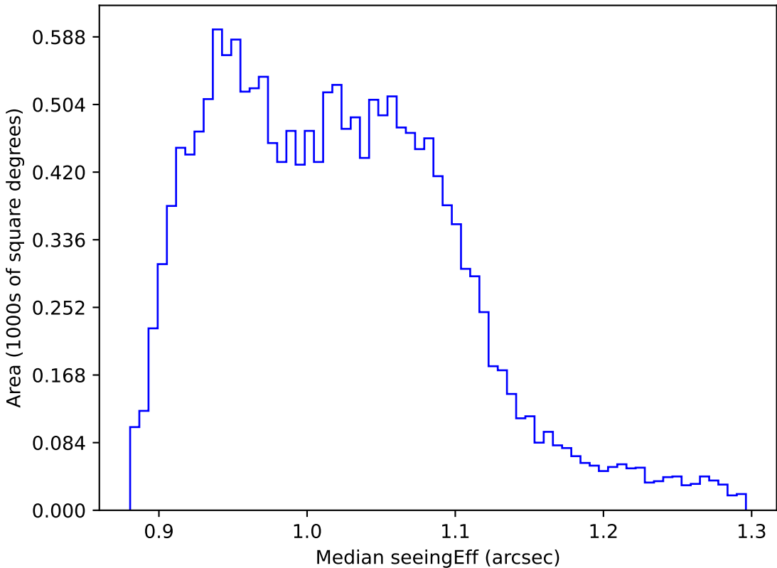
weather_cloudso1v3.4_10yrs WFD r band: Median seeingEff
