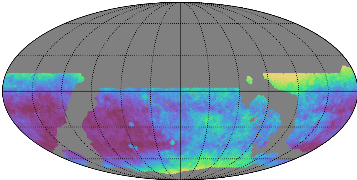
weather_cloudso1v3.4_10yrs WFD i band: Median seeingEff
