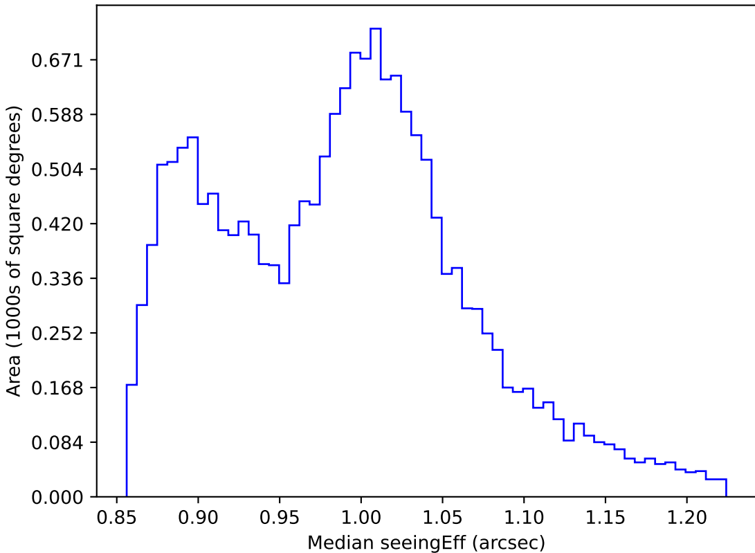
weather_cloudso1v3.4_10yrs WFD i band: Median seeingEff
