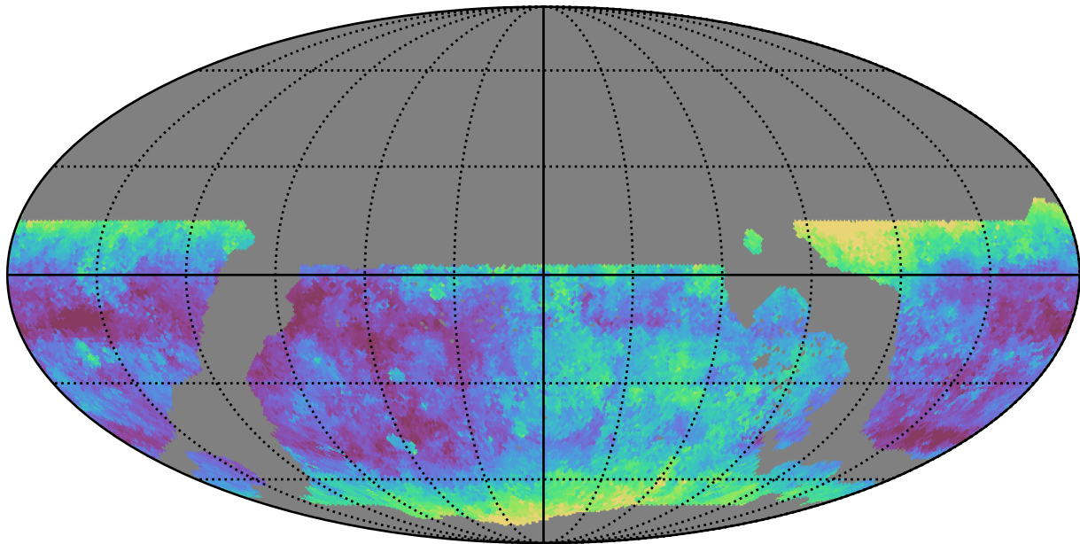
weather_cloudso1v3.4_10yrs WFD g band: Median seeingEff
