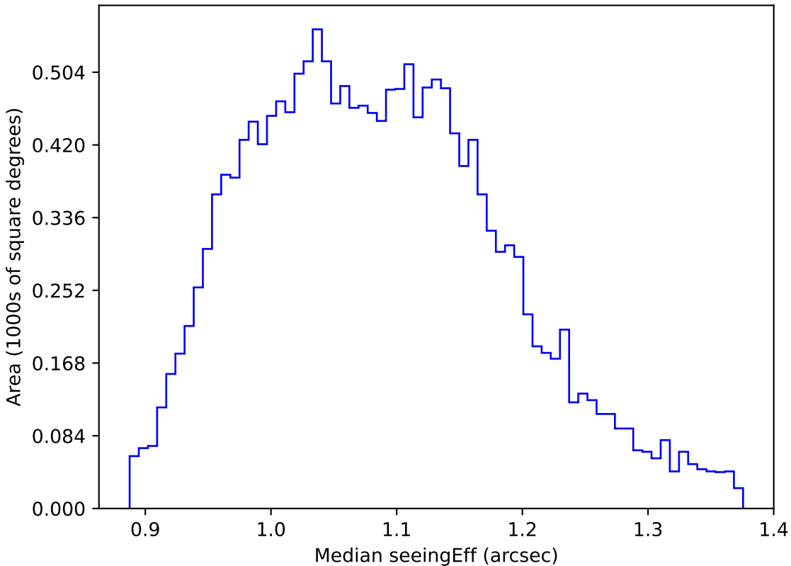
weather_cloudso1v3.4_10yrs WFD g band: Median seeingEff
