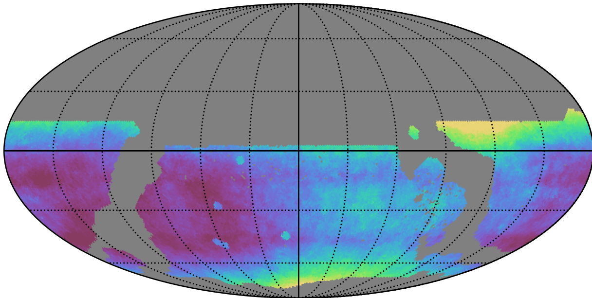
weather_cloudso1v3.4_10yrs WFD all bands: Median seeingEff
