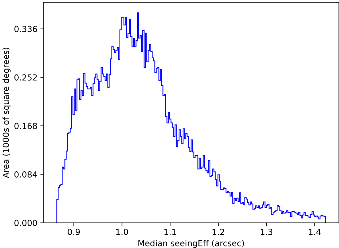
weather_cloudso1v3.4_10yrs All sky z band: Median seeingEff
