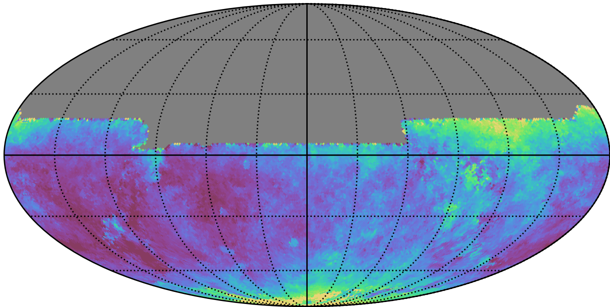
weather_cloudso1v3.4_10yrs All sky y band: Median seeingEff
