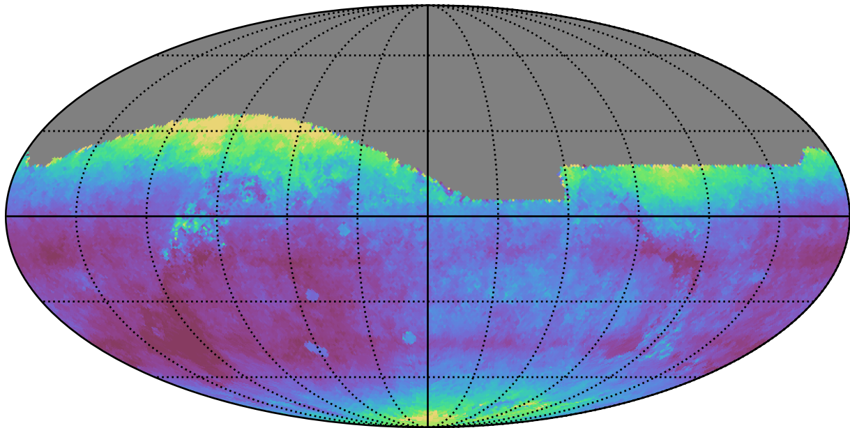
weather_cloudso1v3.4_10yrs All sky r band: Median seeingEff
