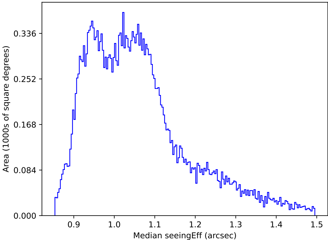
weather_cloudso1v3.4_10yrs All sky r band: Median seeingEff
