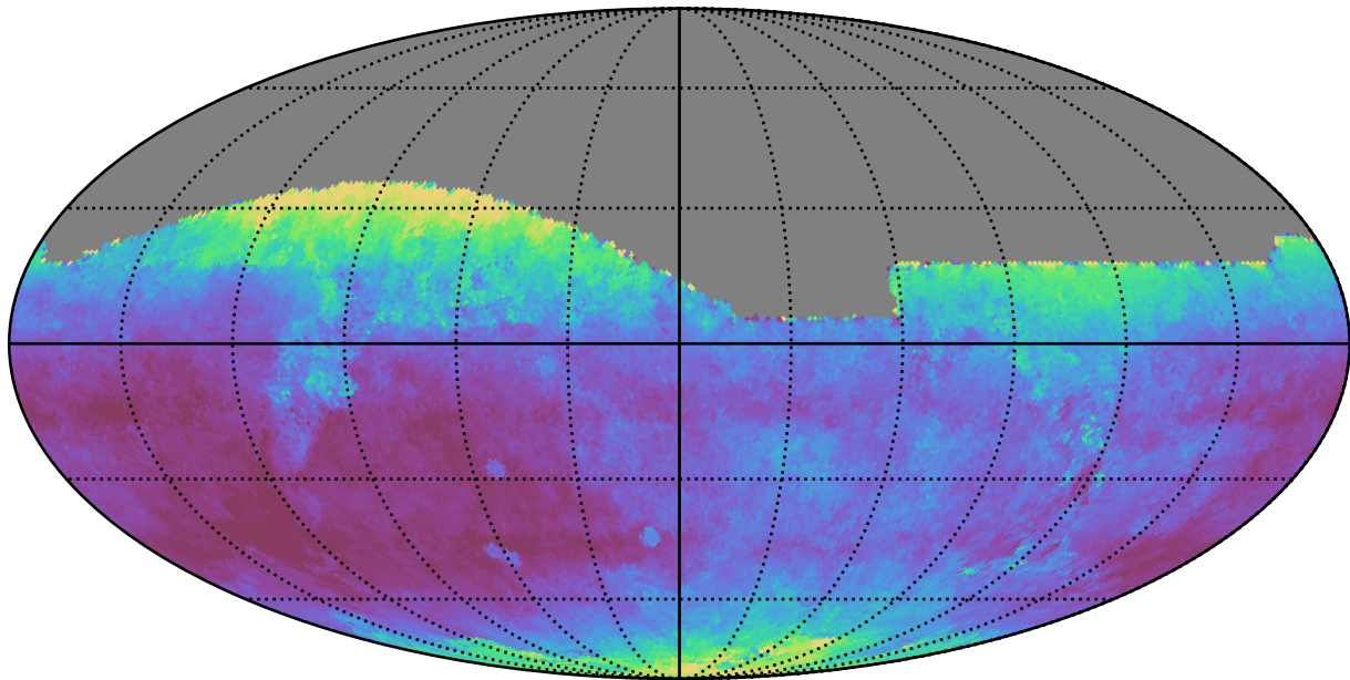
weather_cloudso1v3.4_10yrs All sky i band: Median seeingEff
