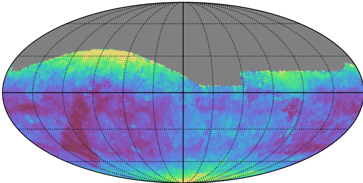
weather_cloudso1v3.4_10yrs All sky g band: Median seeingEff
