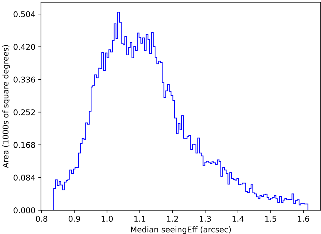
weather_cloudso1v3.4_10yrs All sky g band: Median seeingEff
