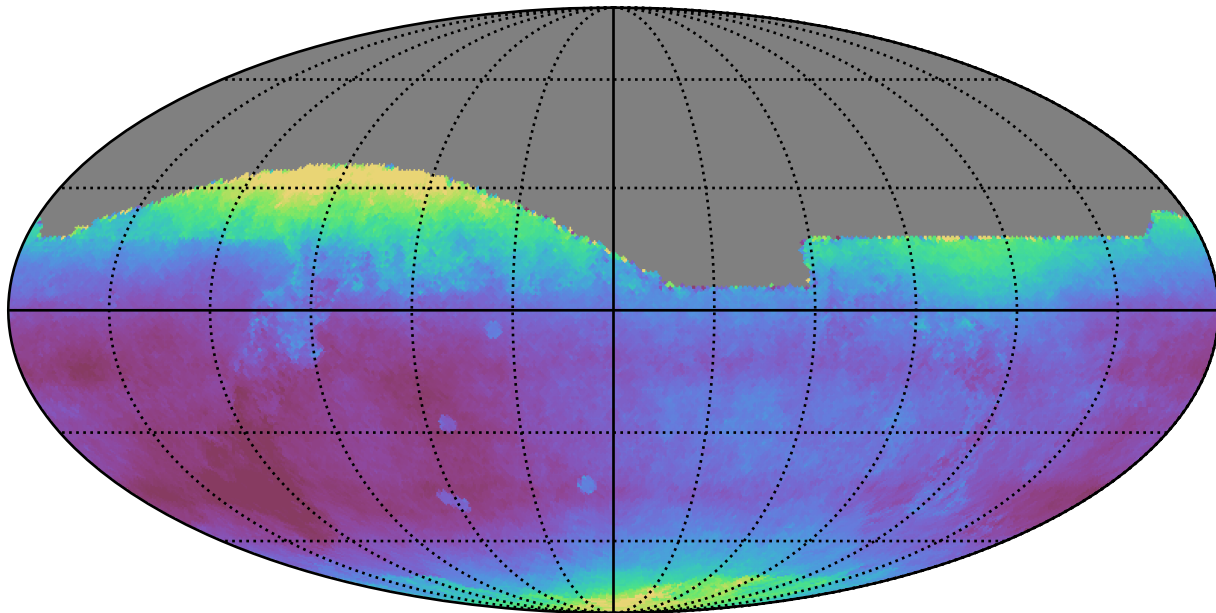
weather_cloudso1v3.4_10yrs All sky all bands: Median seeingEff
