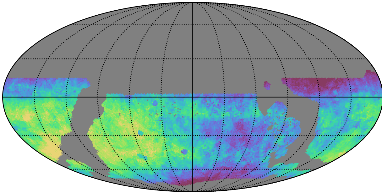
weather_cloudso1v3.4_10yrs WFD z band: Median saturation_mag
