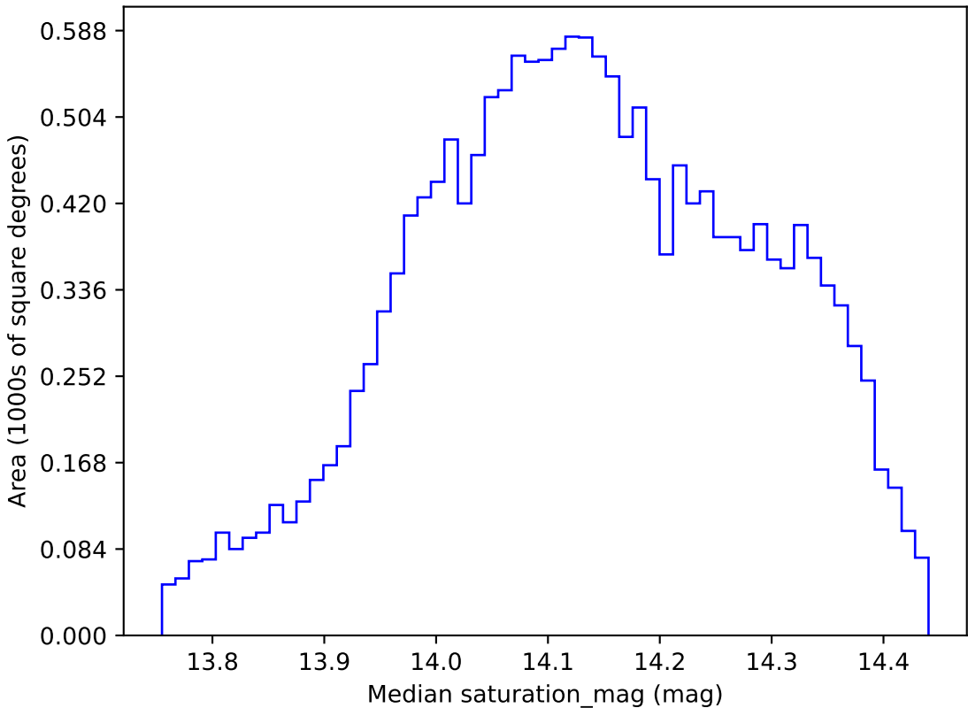
weather_cloudso1v3.4_10yrs WFD z band: Median saturation_mag
