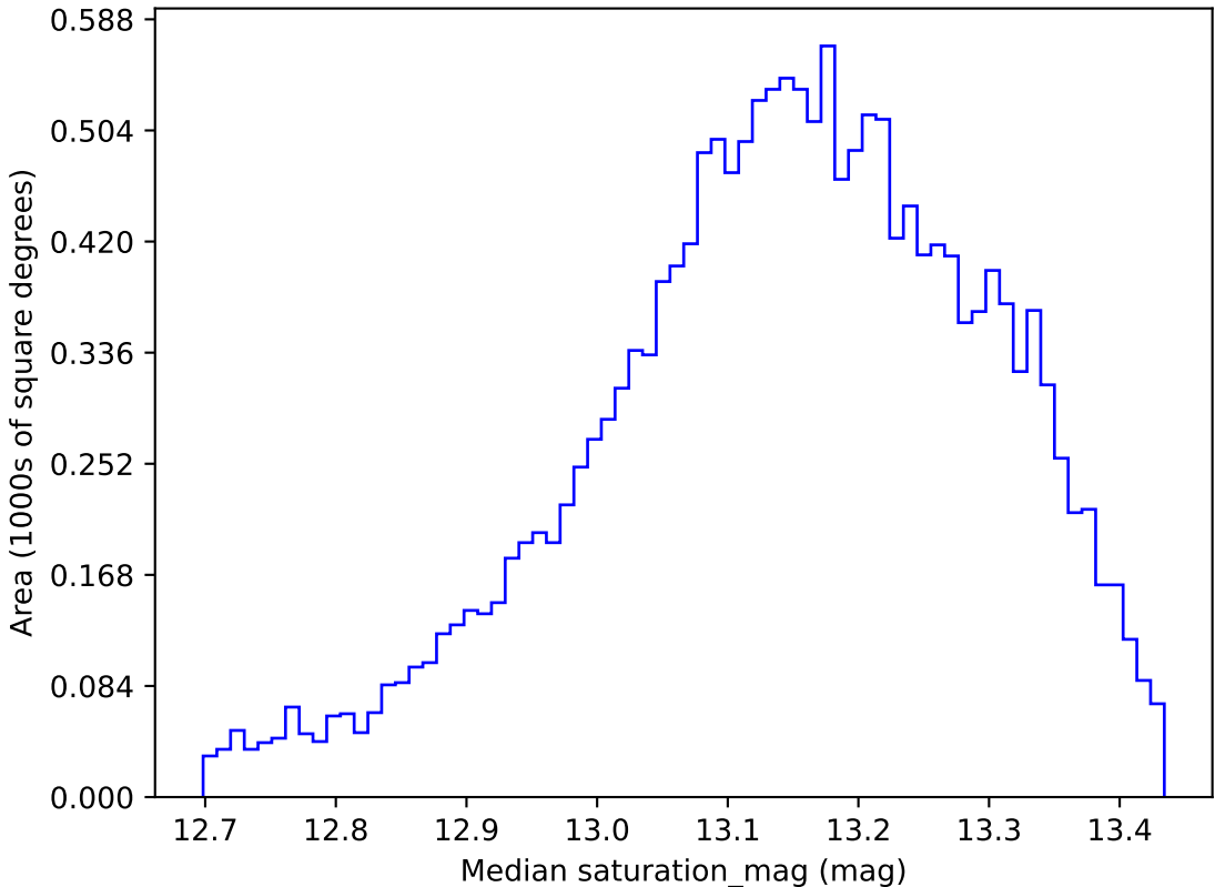
weather_cloudso1v3.4_10yrs WFD y band: Median saturation_mag
