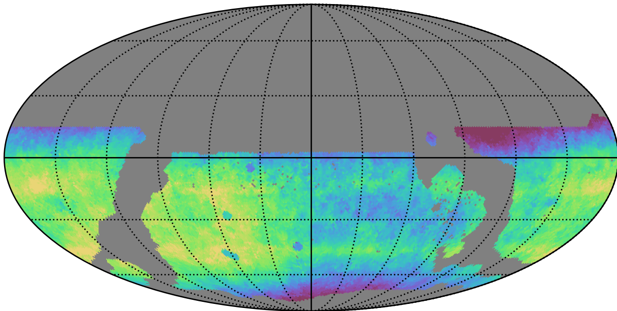
weather_cloudso1v3.4_10yrs WFD r band: Median saturation_mag
