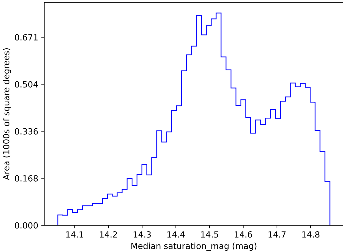
weather_cloudso1v3.4_10yrs WFD i band: Median saturation_mag
