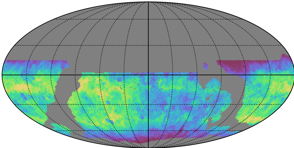
weather_cloudso1v3.4_10yrs WFD g band: Median saturation_mag
