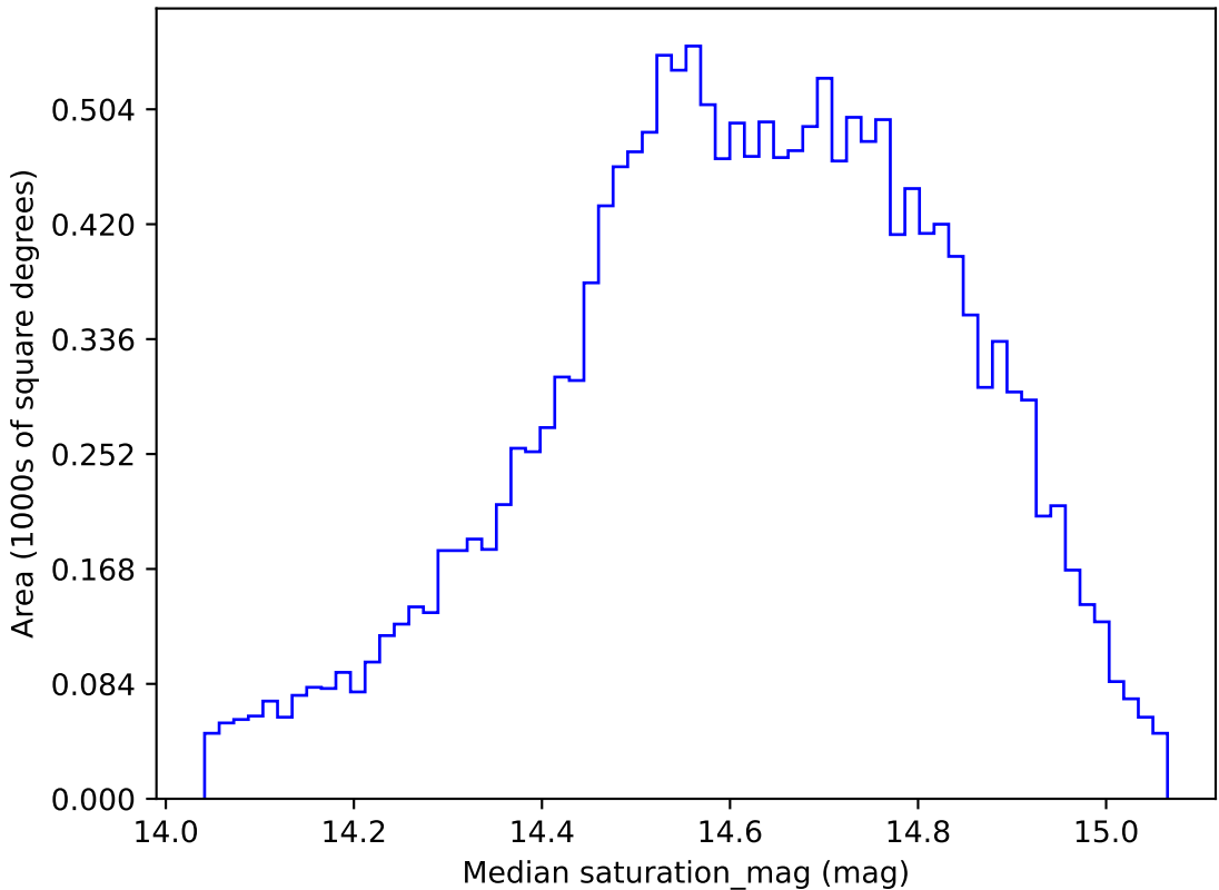
weather_cloudso1v3.4_10yrs WFD g band: Median saturation_mag
