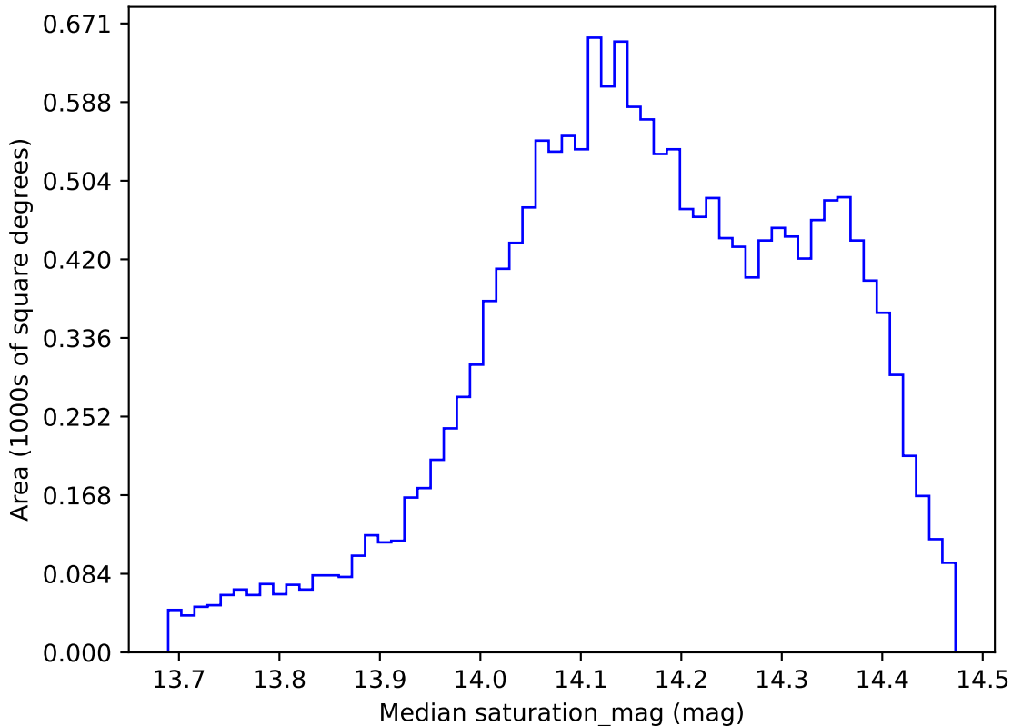
weather_cloudso1v3.4_10yrs WFD all bands: Median saturation_mag
