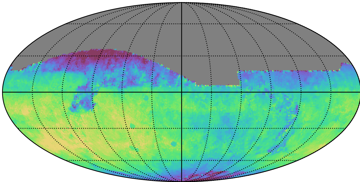
weather_cloudso1v3.4_10yrs All sky z band: Median saturation_mag
