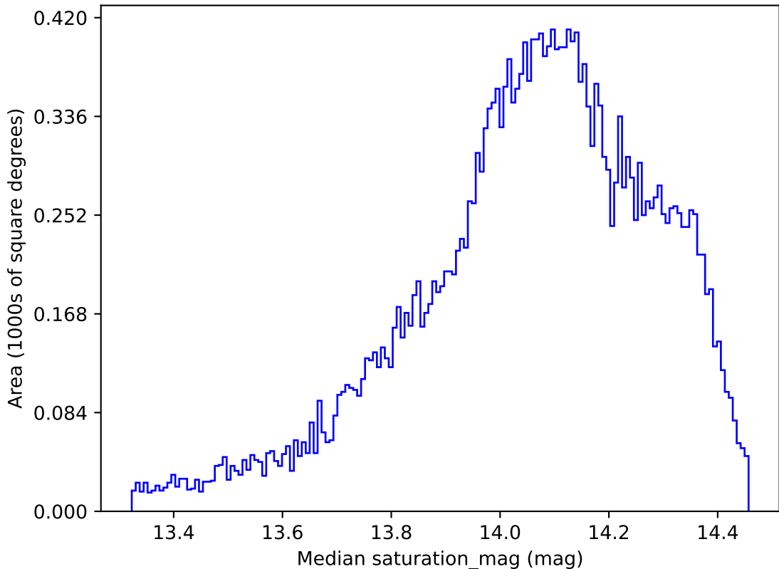
weather_cloudso1v3.4_10yrs All sky z band: Median saturation_mag
