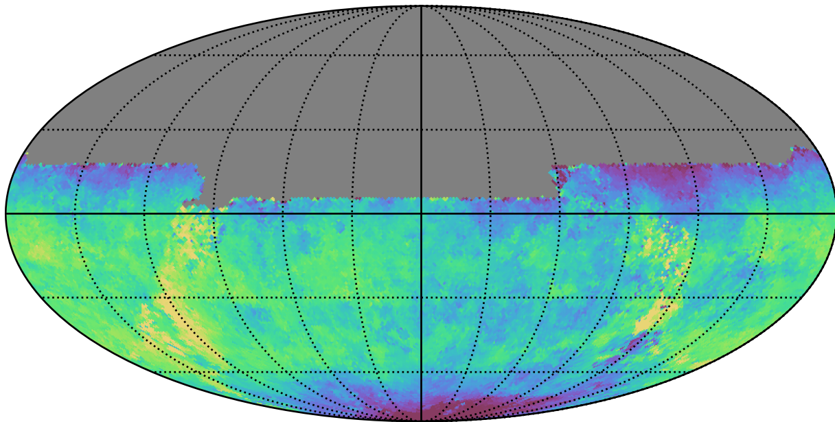
weather_cloudso1v3.4_10yrs All sky u band: Median saturation_mag
