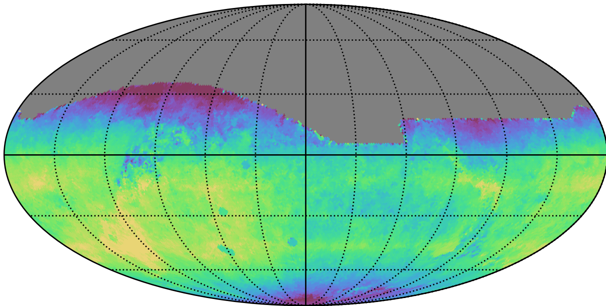
weather_cloudso1v3.4_10yrs All sky r band: Median saturation_mag
