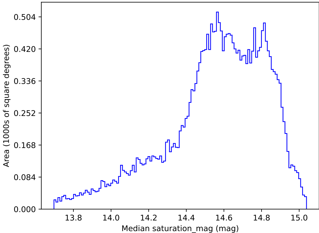
weather_cloudso1v3.4_10yrs All sky r band: Median saturation_mag
