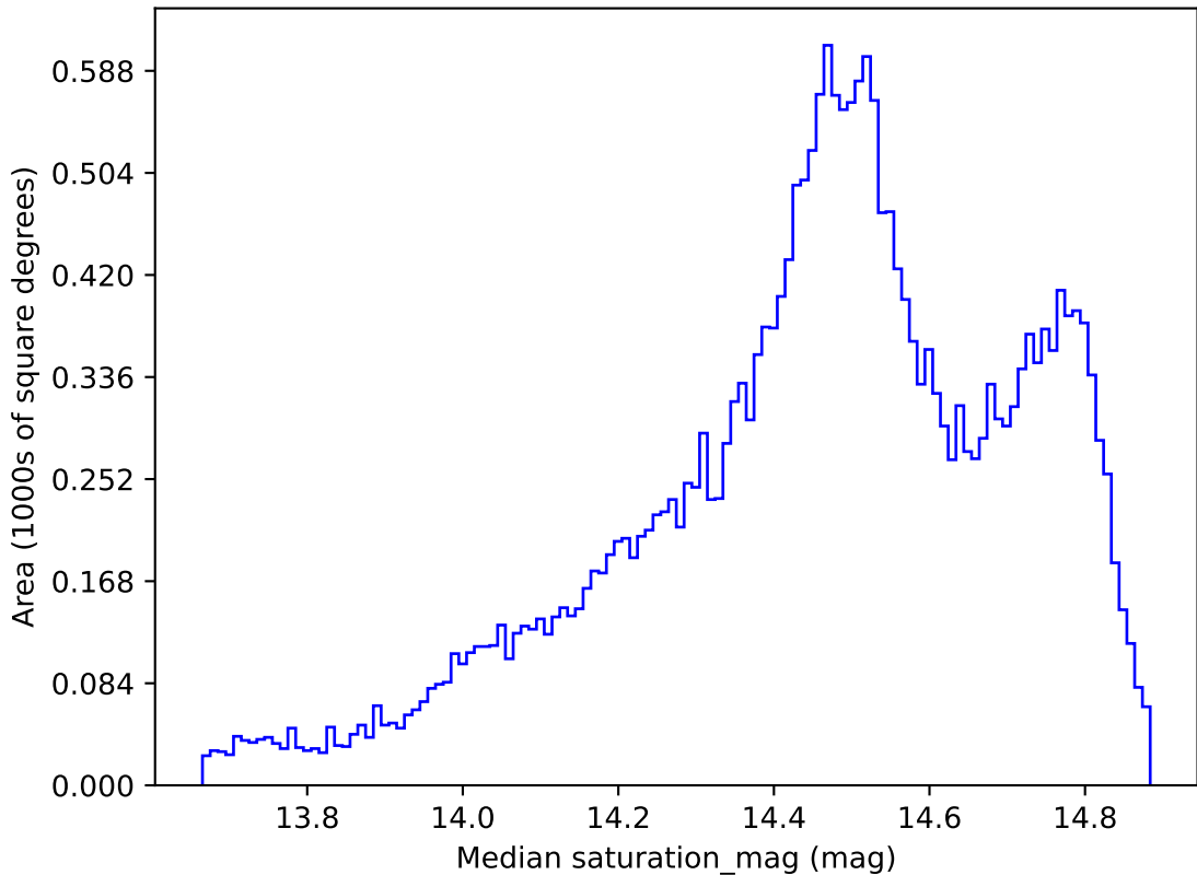
weather_cloudso1v3.4_10yrs All sky i band: Median saturation_mag
