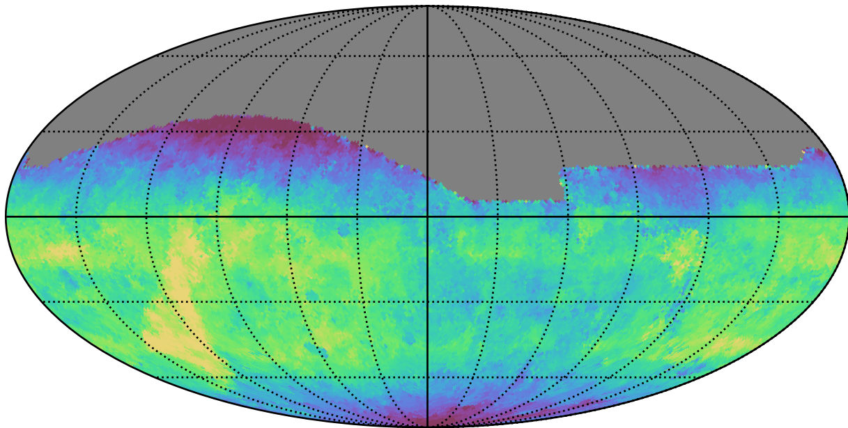
weather_cloudso1v3.4_10yrs All sky g band: Median saturation_mag
