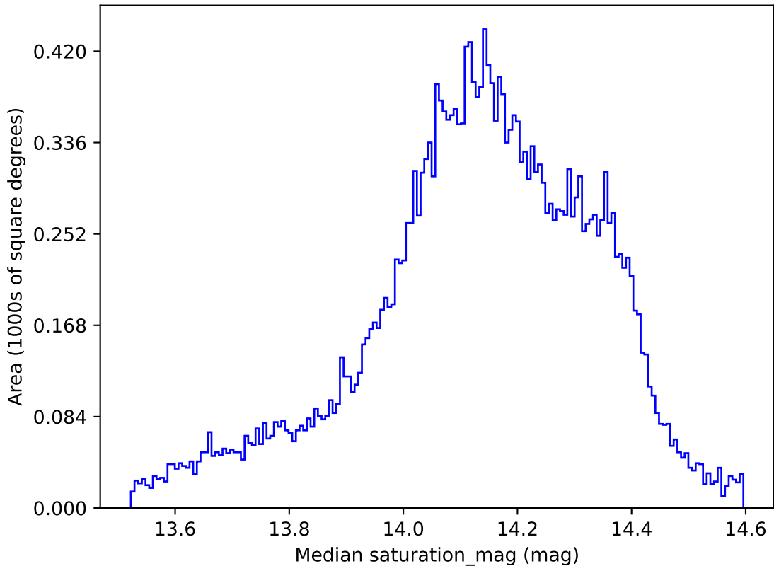
weather_cloudso1v3.4_10yrs All sky all bands: Median saturation_mag
