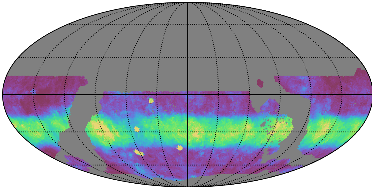
weather_cloudso1v3.4_10yrs WFD z band: Median normairmass
