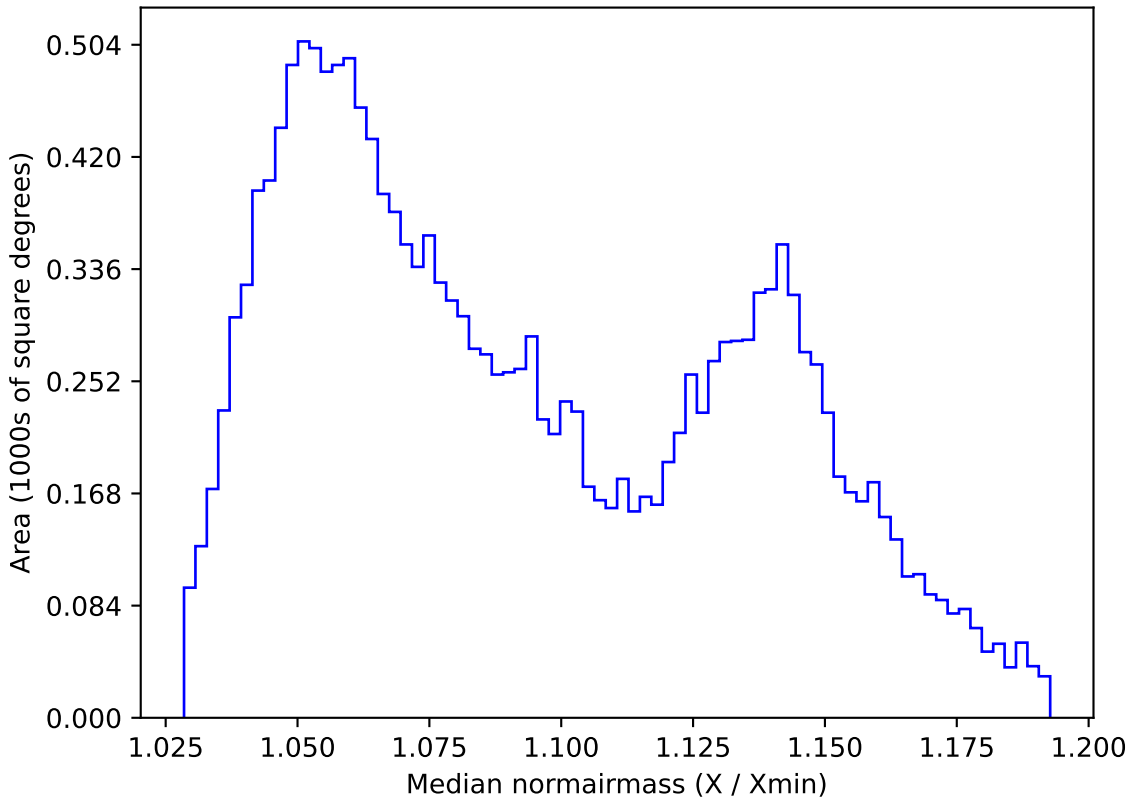
weather_cloudso1v3.4_10yrs WFD y band: Median normairmass
