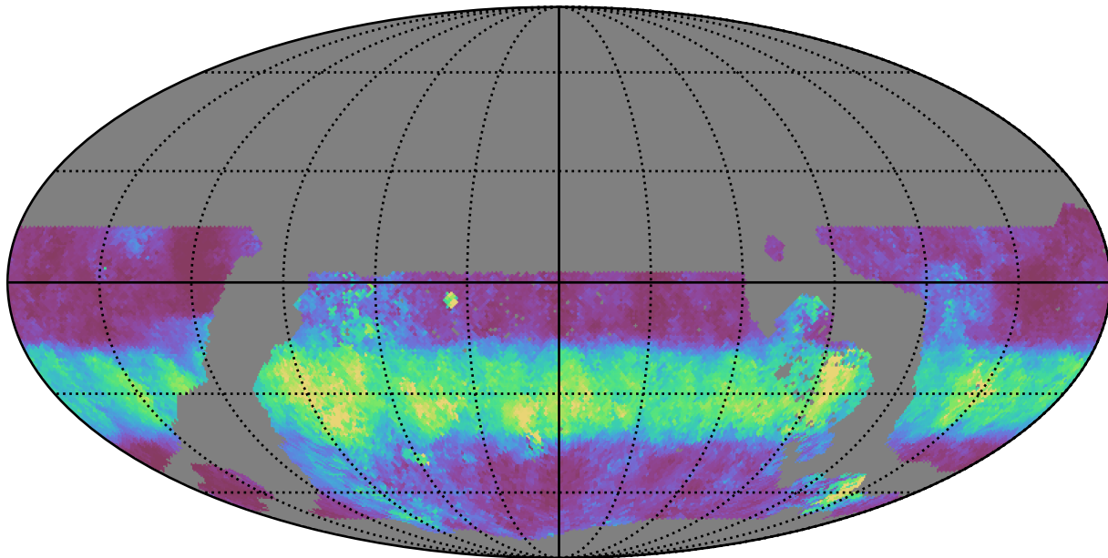
weather_cloudso1v3.4_10yrs WFD u band: Median normairmass
