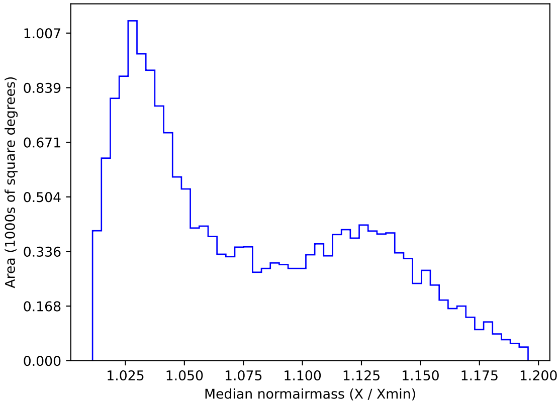
weather_cloudso1v3.4_10yrs WFD u band: Median normairmass
