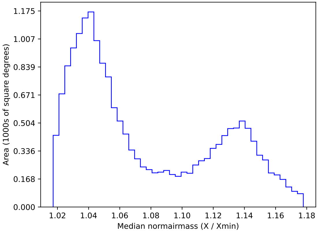
weather_cloudso1v3.4_10yrs WFD r band: Median normairmass
