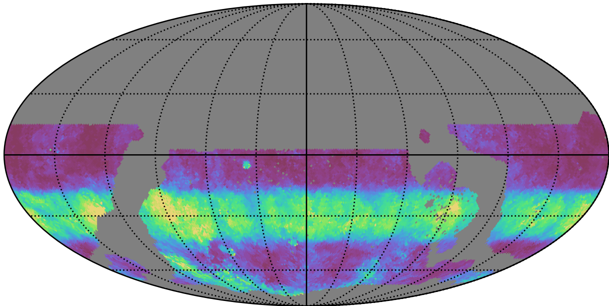
weather_cloudso1v3.4_10yrs WFD g band: Median normairmass
