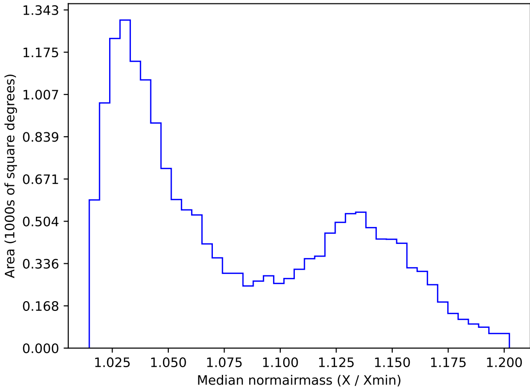
weather_cloudso1v3.4_10yrs WFD g band: Median normairmass
