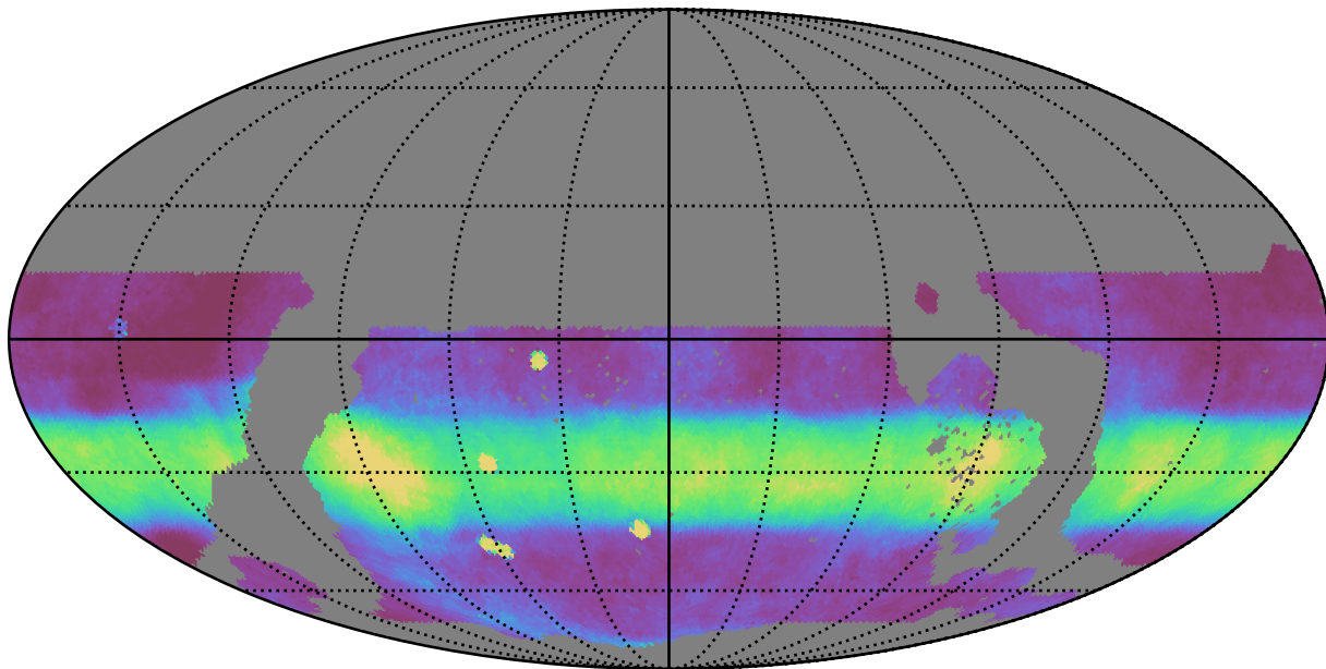
weather_cloudso1v3.4_10yrs WFD all bands: Median normairmass
