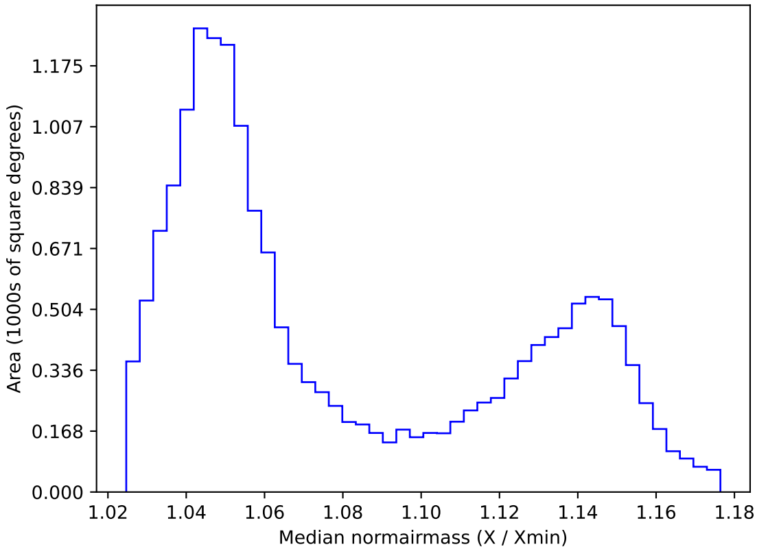
weather_cloudso1v3.4_10yrs WFD all bands: Median normairmass
