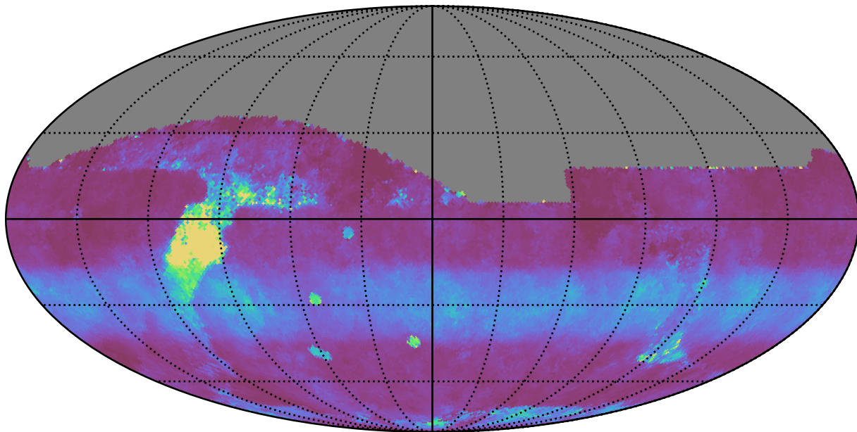
weather_cloudso1v3.4_10yrs All sky z band: Median normairmass
