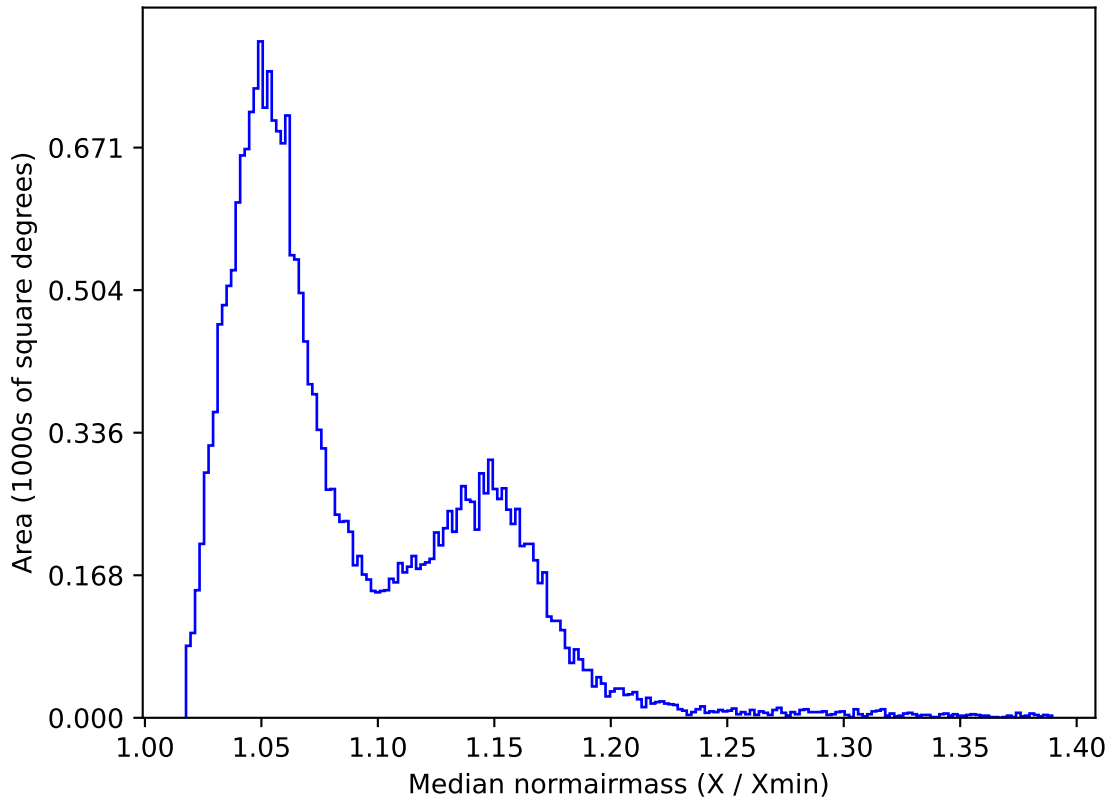
weather_cloudso1v3.4_10yrs All sky z band: Median normairmass
