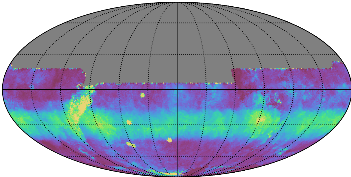
weather_cloudso1v3.4_10yrs All sky y band: Median normairmass
