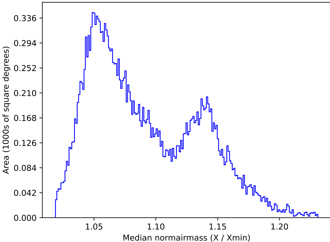
weather_cloudso1v3.4_10yrs All sky y band: Median normairmass
