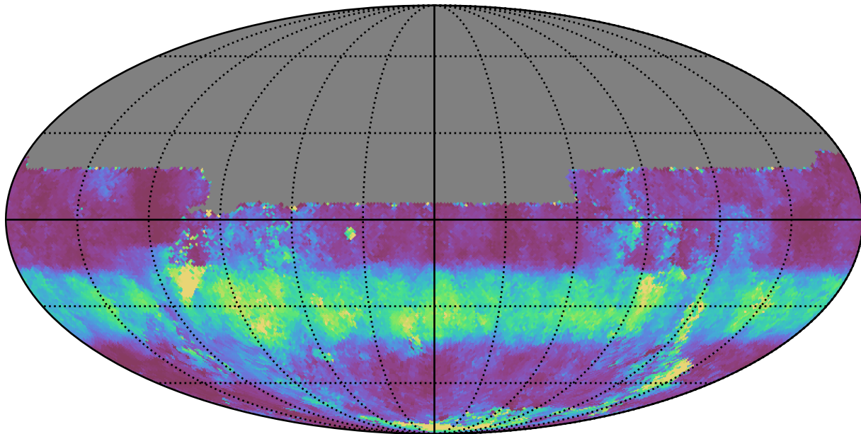
weather_cloudso1v3.4_10yrs All sky u band: Median normairmass
