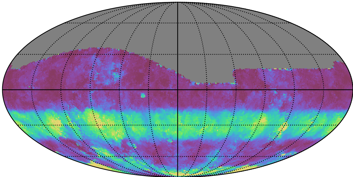
weather_cloudso1v3.4_10yrs All sky g band: Median normairmass
