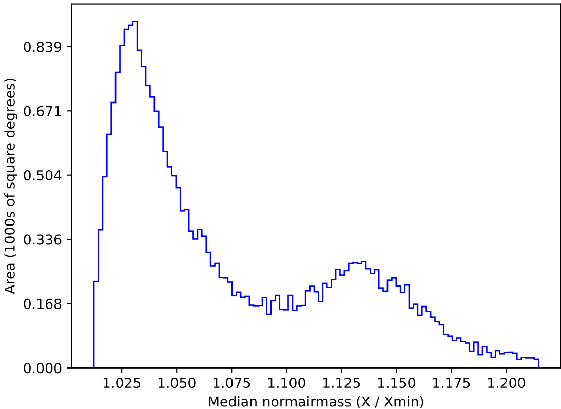
weather_cloudso1v3.4_10yrs All sky g band: Median normairmass
