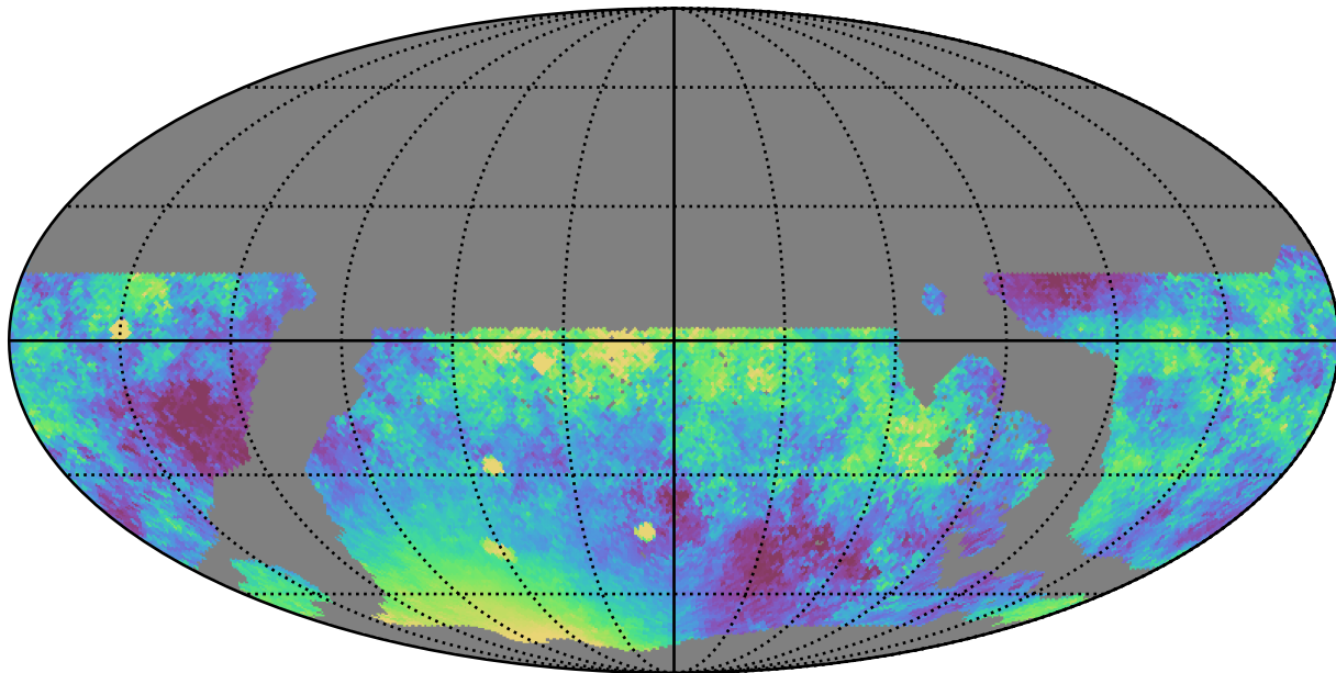
weather_cloudso1v3.4_10yrs WFD z band: Median moonDistance
