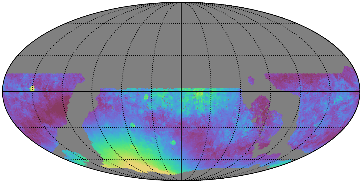
weather_cloudso1v3.4_10yrs WFD y band: Median moonDistance
