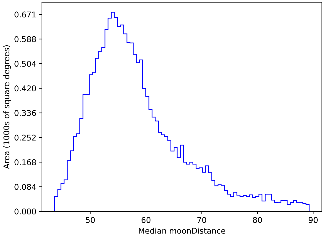
weather_cloudso1v3.4_10yrs WFD y band: Median moonDistance
